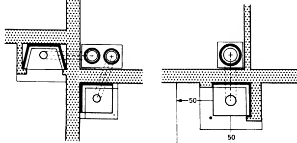
③ Fireplaces open on one/two sides in separate rooms ④ Fireplace open on two sides with safety area
